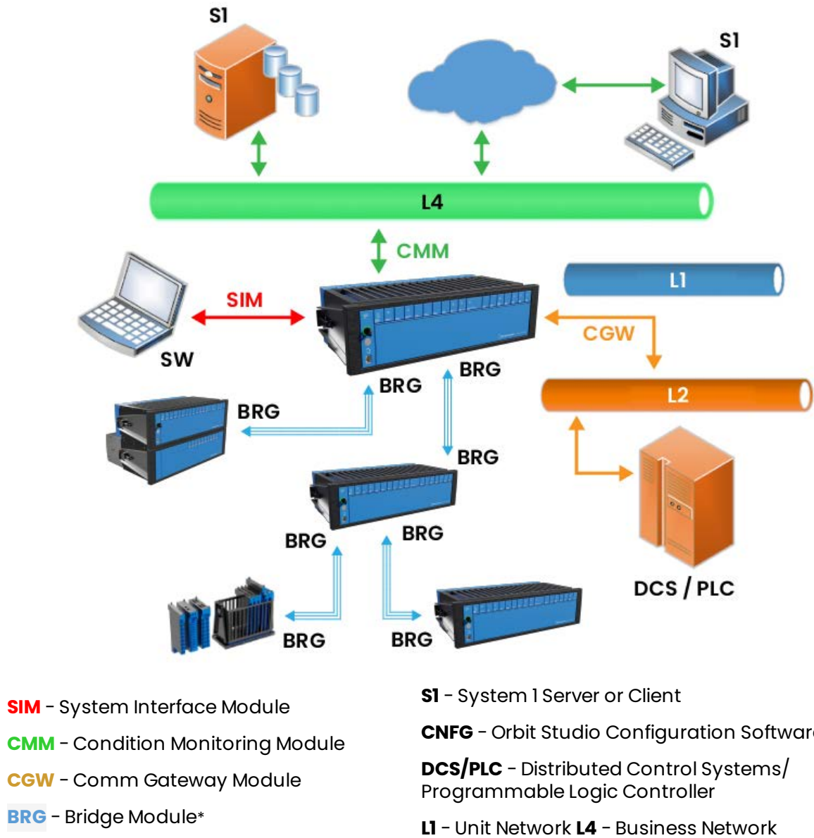
Figure 1: System Diagram
